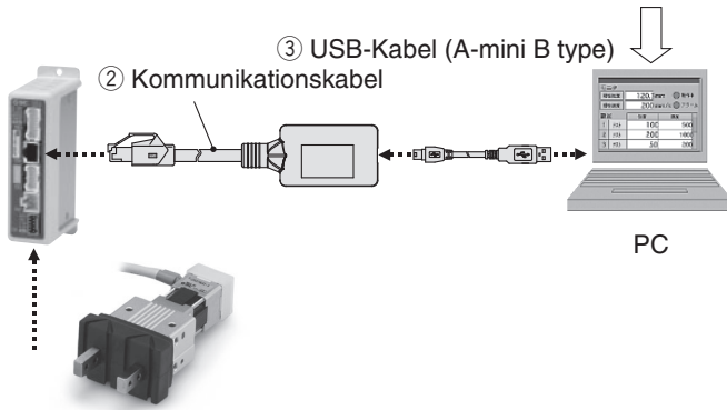
① Controller-Einstellsoftware
